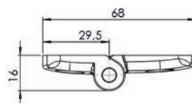
Charnière Al 40x30 E=40mm
