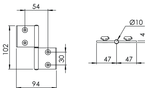
Kit charnière 45x45 Al PP0
