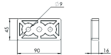
Plaque de base 8 90x45 M12, ep 16mm, noir
