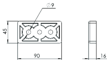
Plaque de base 8 90x45 M10, ep 16 mm, noir
